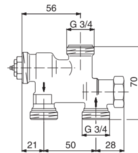
Dimensions of valve for "TKM" system (one/two pipe)
